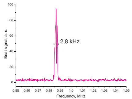
Beats between two identical TIS-SF-777 lasers detected by a avalanche photodiode and introduced into rf spectrum analyzer (1-s sweep time in the range of 100 kHz)
